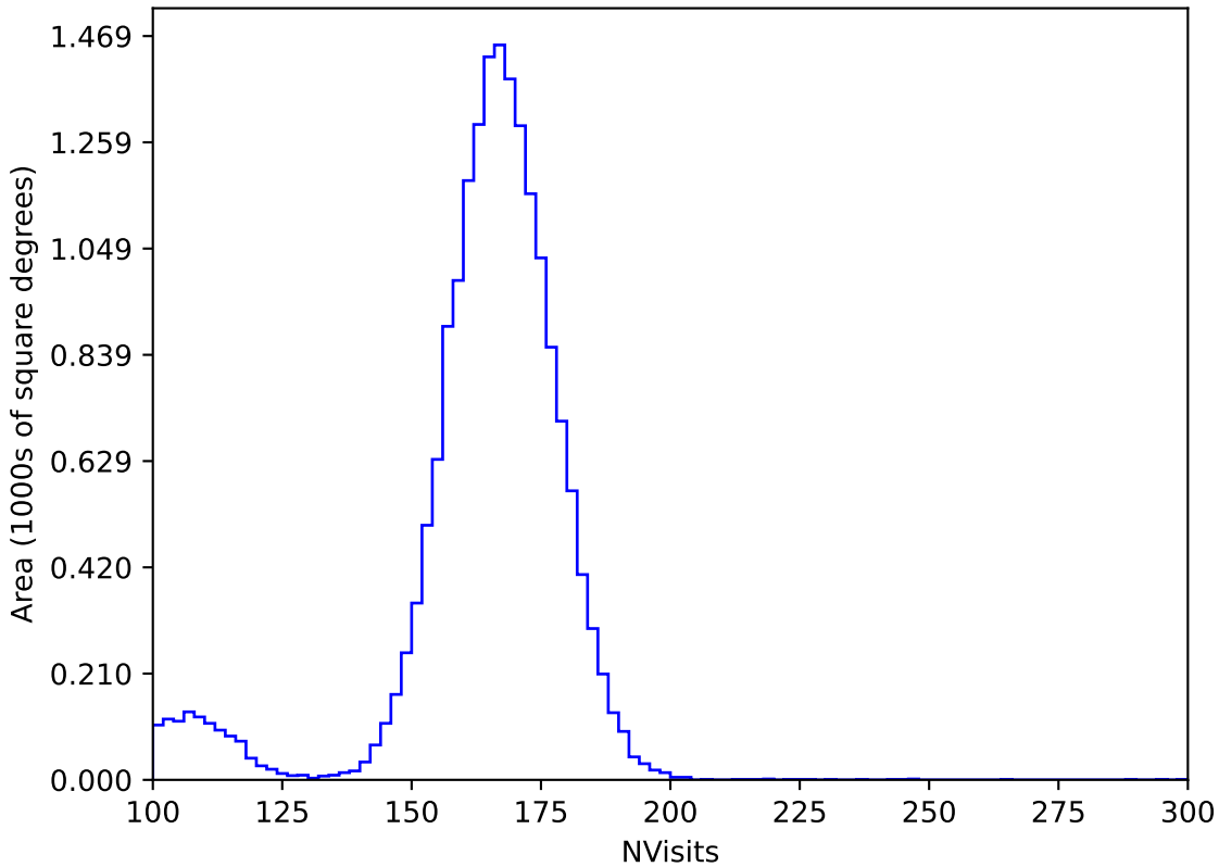
noroll_mjdp365_v3.4_10yrs WFD y band: NVisits
