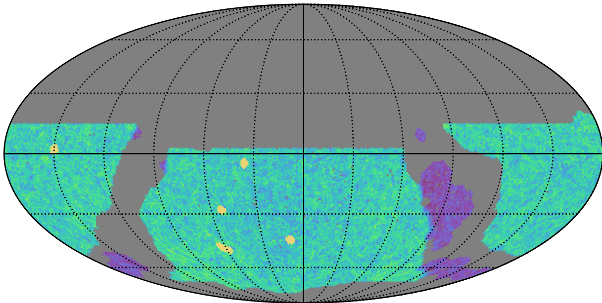
noroll_mjdp365_v3.4_10yrs WFD u band: NVisits
