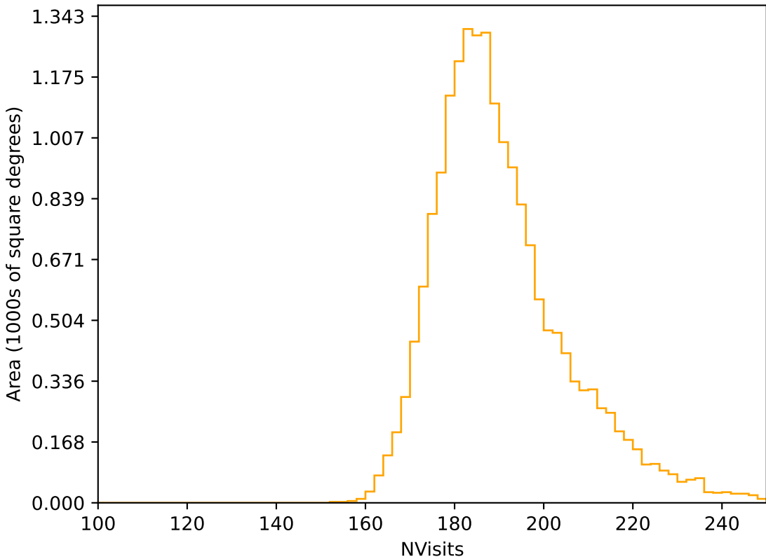
noroll_mjdp365_v3.4_10yrs WFD r band: NVisits
