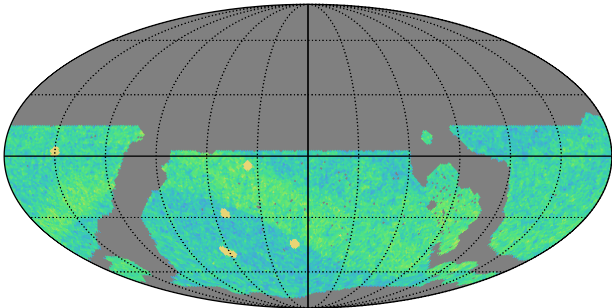
noroll_mjdp365_v3.4_10yrs WFD i band: NVisits
