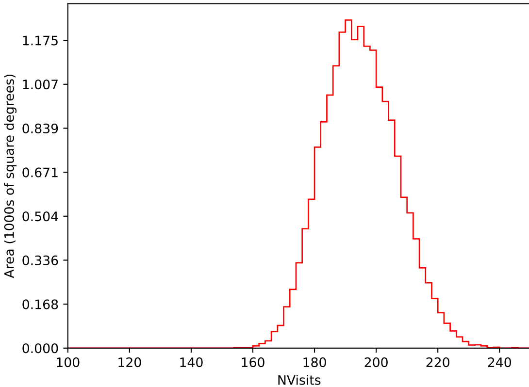
noroll_mjdp365_v3.4_10yrs WFD i band: NVisits
