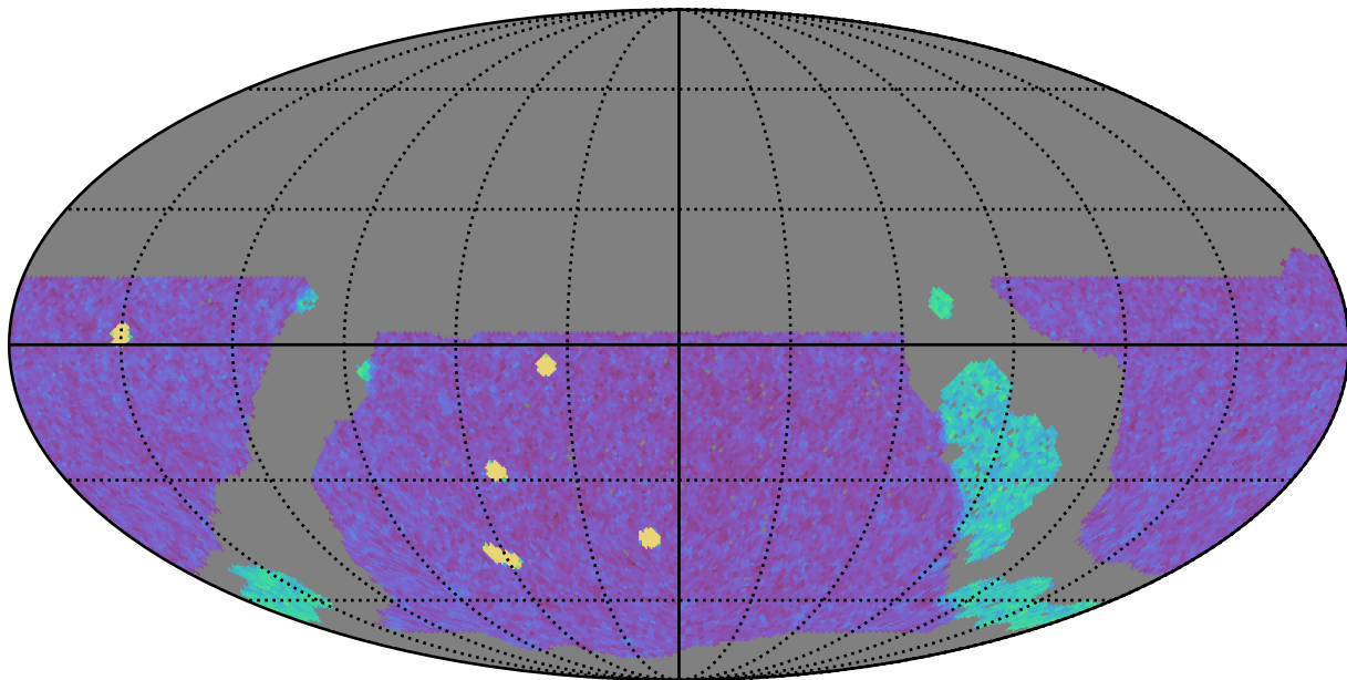
noroll_mjdp365_v3.4_10yrs WFD g band: NVisits
