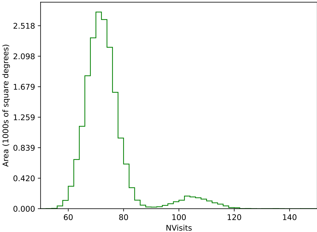
noroll_mjdp365_v3.4_10yrs WFD g band: NVisits
