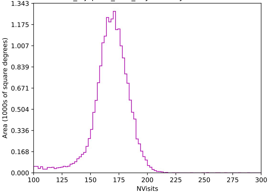
noroll_mjdp365_v3.4_10yrs All sky z band: NVisits
