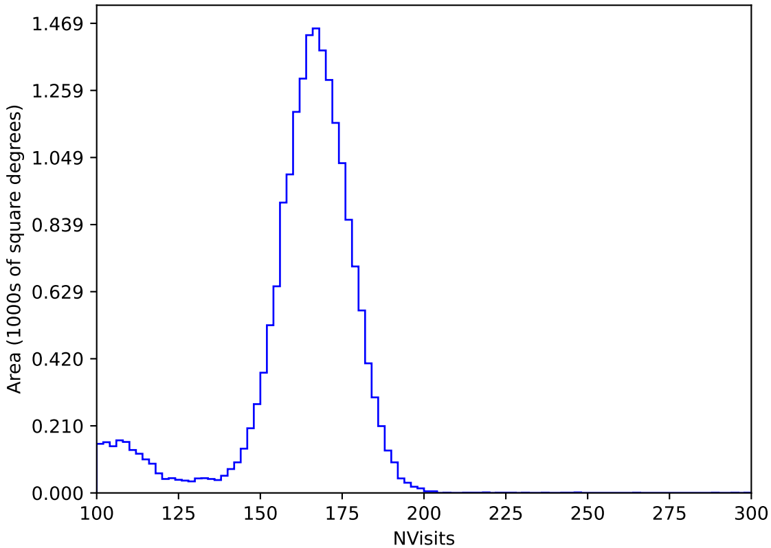
noroll_mjdp365_v3.4_10yrs All sky y band: NVisits
