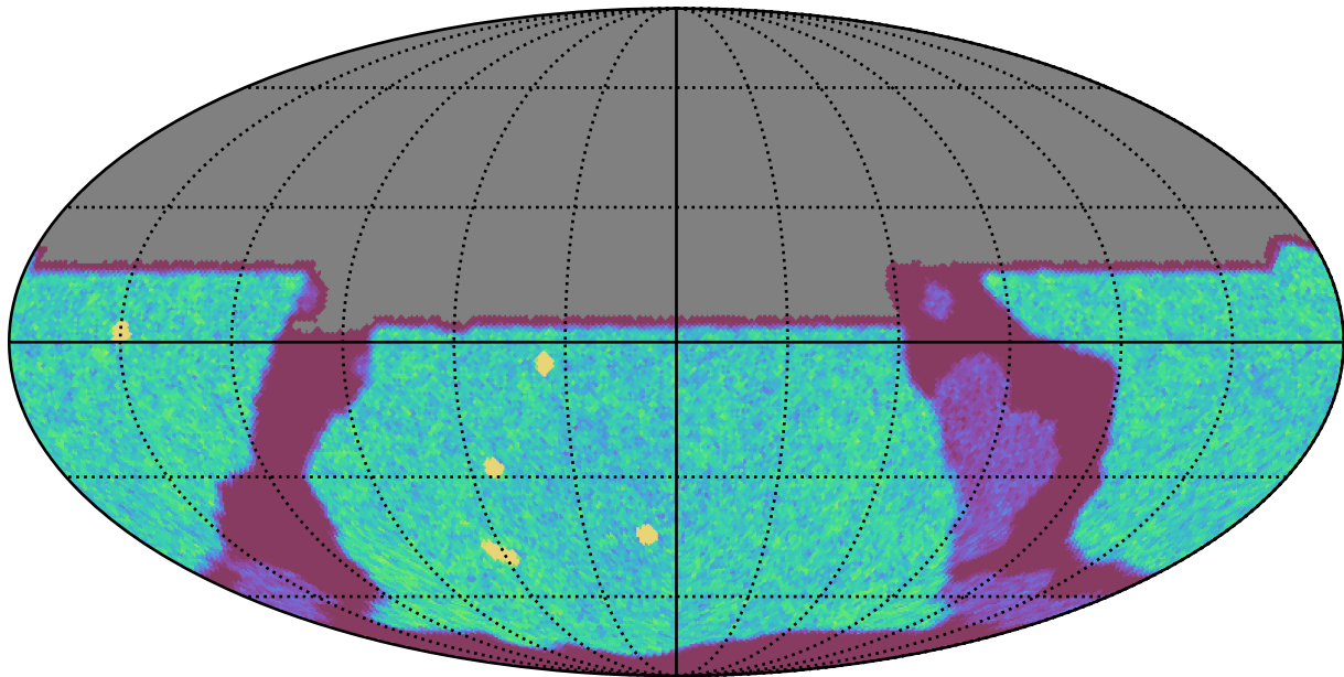
noroll_mjdp365_v3.4_10yrs All sky u band: NVisits
