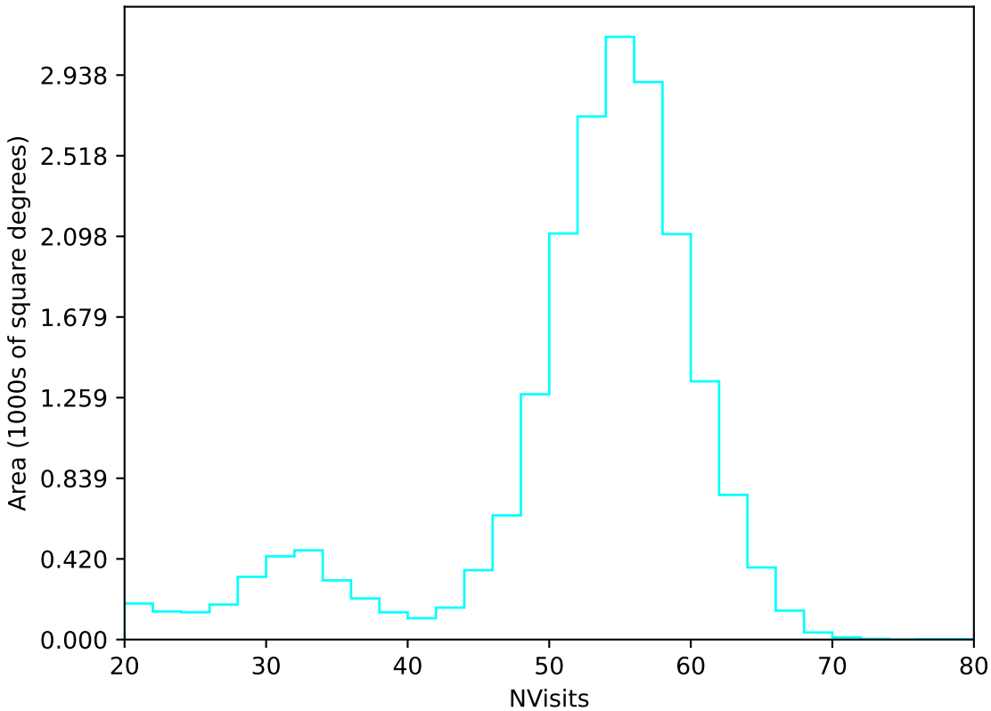
noroll_mjdp365_v3.4_10yrs All sky u band: NVisits
