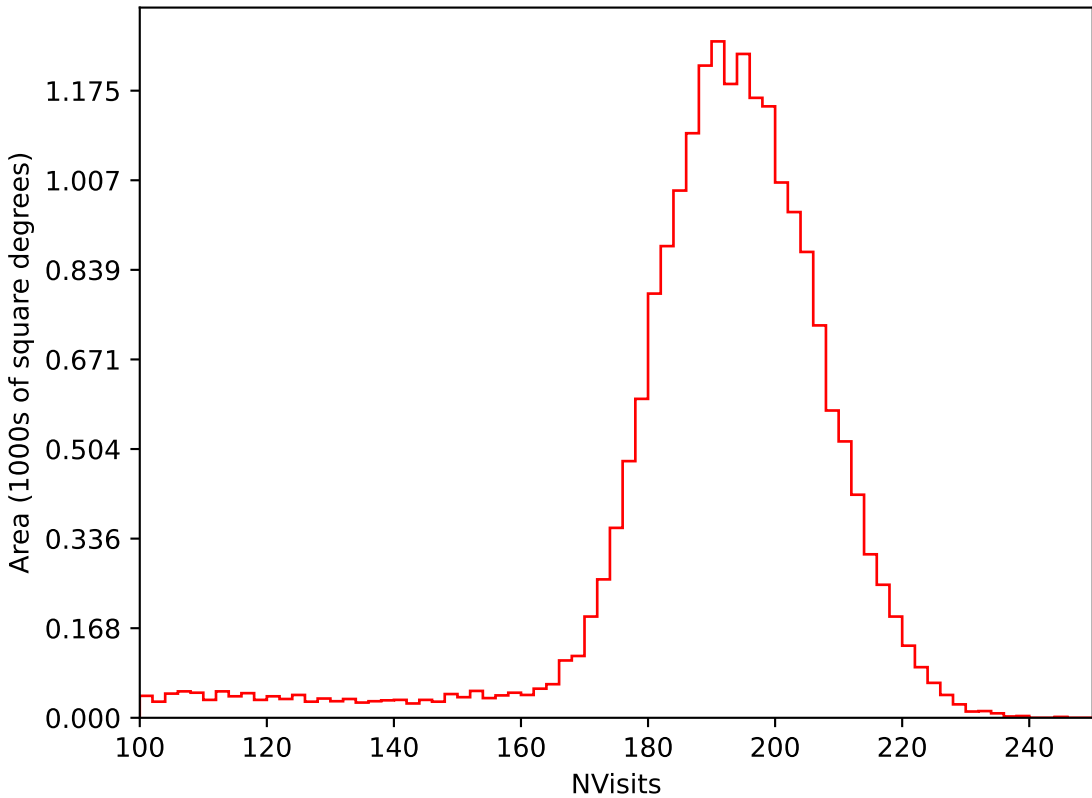
noroll_mjdp365_v3.4_10yrs All sky i band: NVisits
