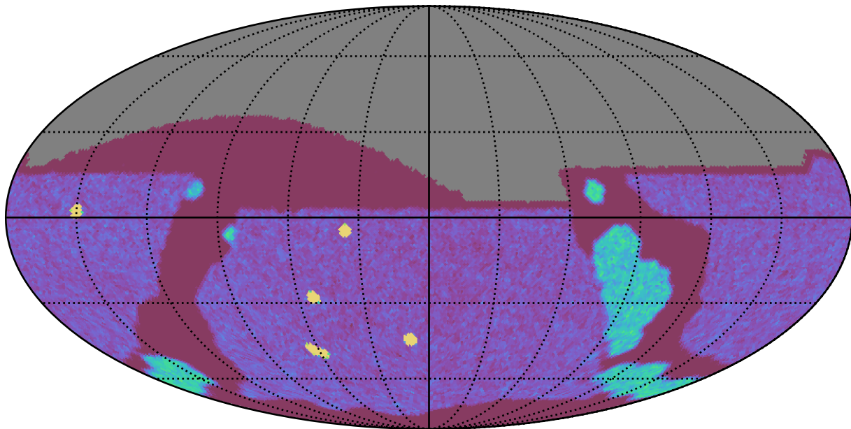
noroll_mjdp365_v3.4_10yrs All sky g band: NVisits
