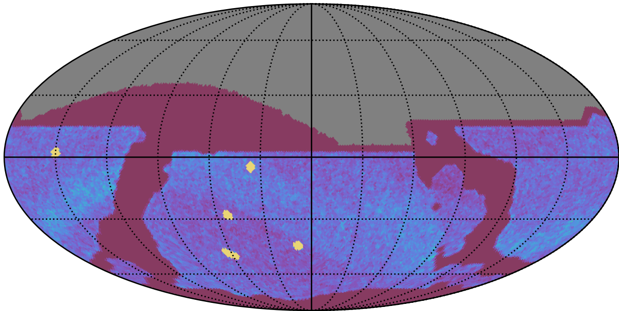
noroll_mjdp365_v3.4_10yrs All sky all bands: NVisits
