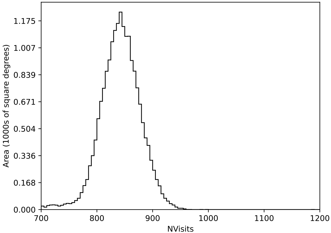
noroll_mjdp365_v3.4_10yrs All sky all bands: NVisits
