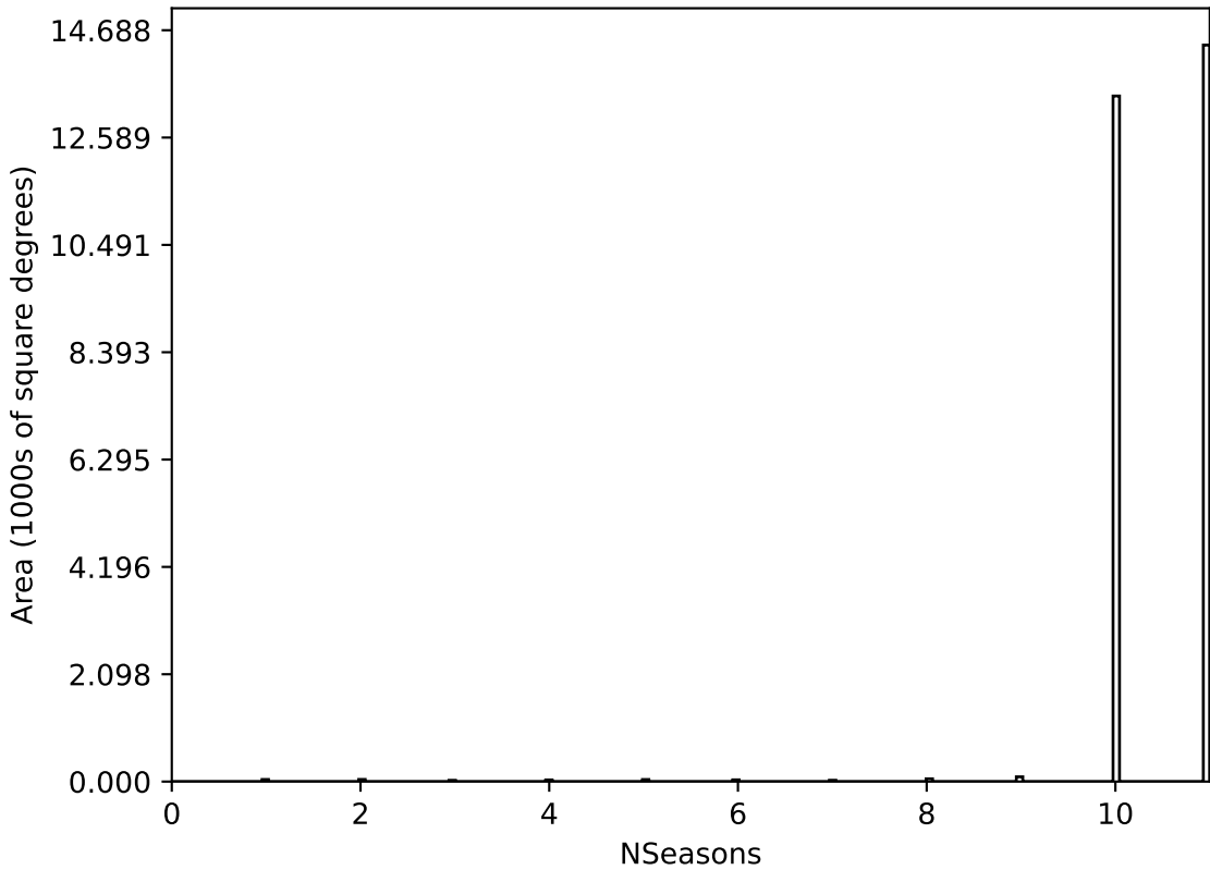
noroll_mjdp365_v3.4_10yrs All sky all bands: NSeasons
