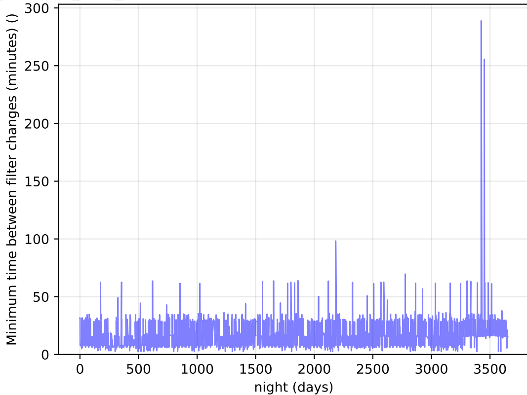
noroll_mjdp365_v3.4_10yrs Per Night: Minimum time between filter changes (minutes)
