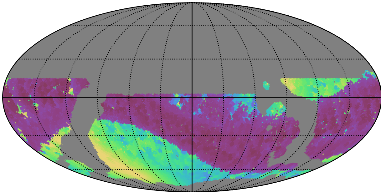
noroll_mjdp365_v3.4_10yrs WFD z band: Min solarElong
