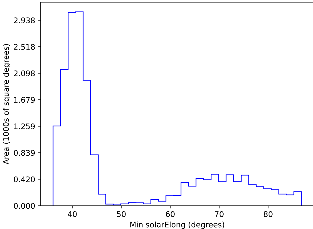
noroll_mjdp365_v3.4_10yrs WFD z band: Min solarElong
