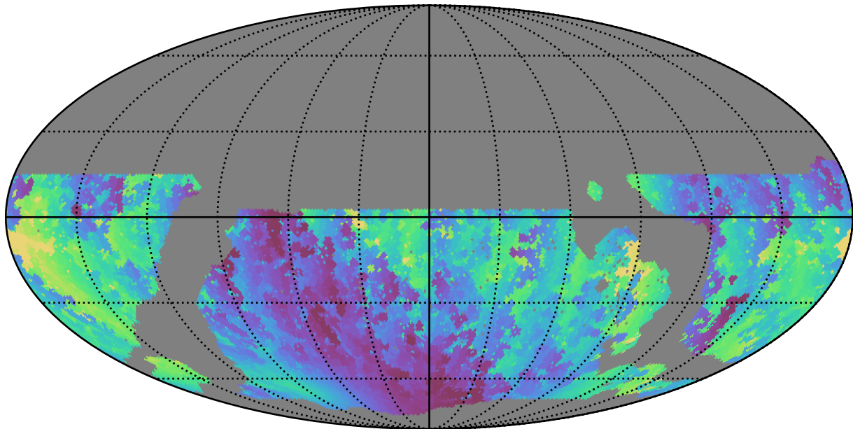
noroll_mjdp365_v3.4_10yrs WFD u band: Min solarElong
