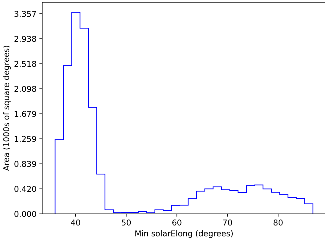
noroll_mjdp365_v3.4_10yrs WFD i band: Min solarElong
