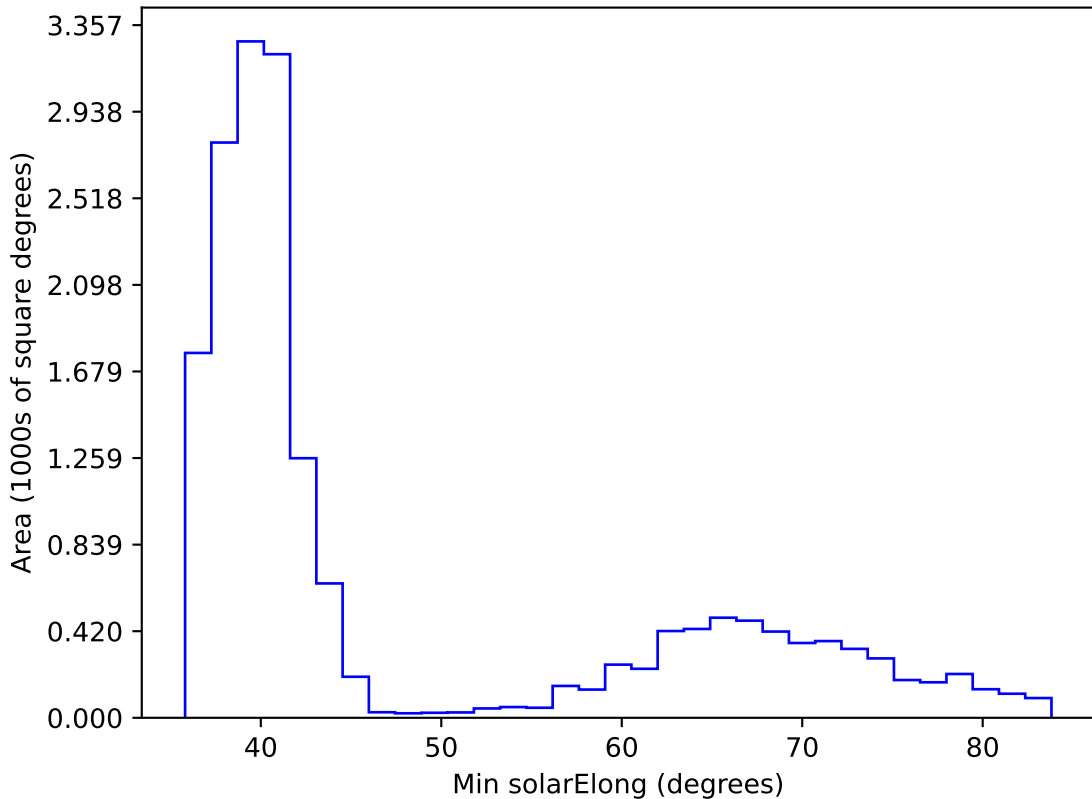
noroll_mjdp365_v3.4_10yrs WFD all bands: Min solarElong
