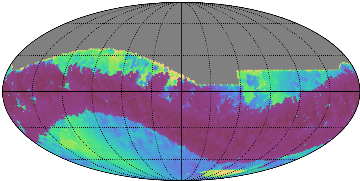
noroll_mjdp365_v3.4_10yrs All sky z band: Min solarElong
