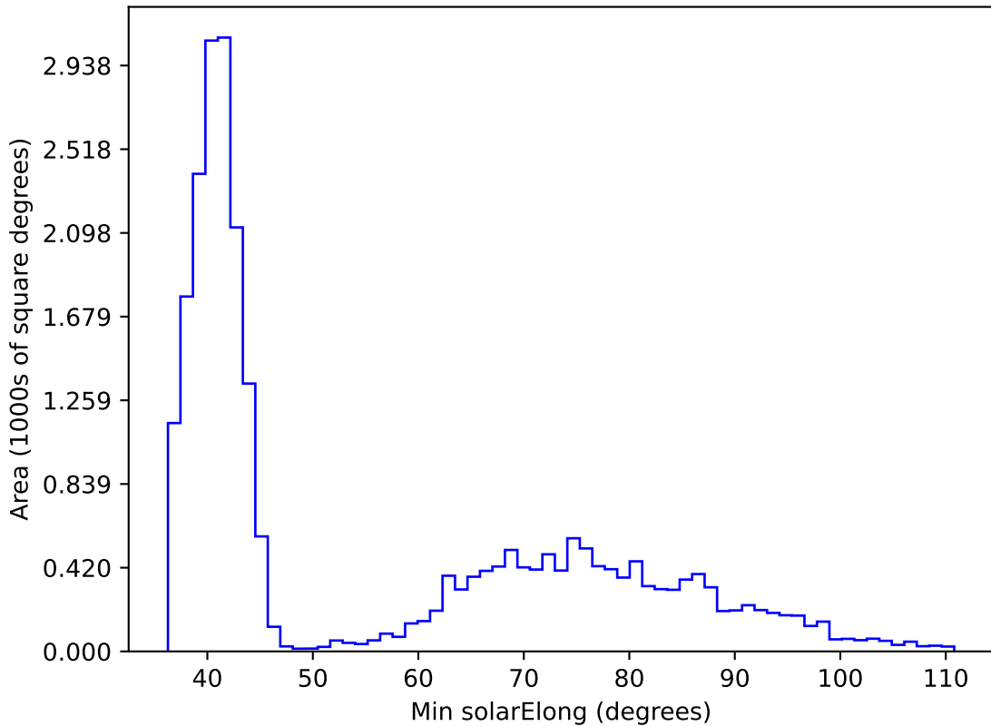
noroll_mjdp365_v3.4_10yrs All sky z band: Min solarElong
