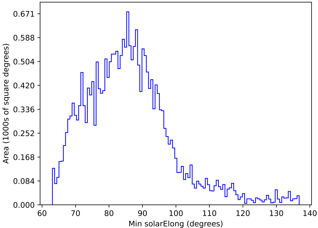
noroll_mjdp365_v3.4_10yrs All sky u band: Min solarElong
