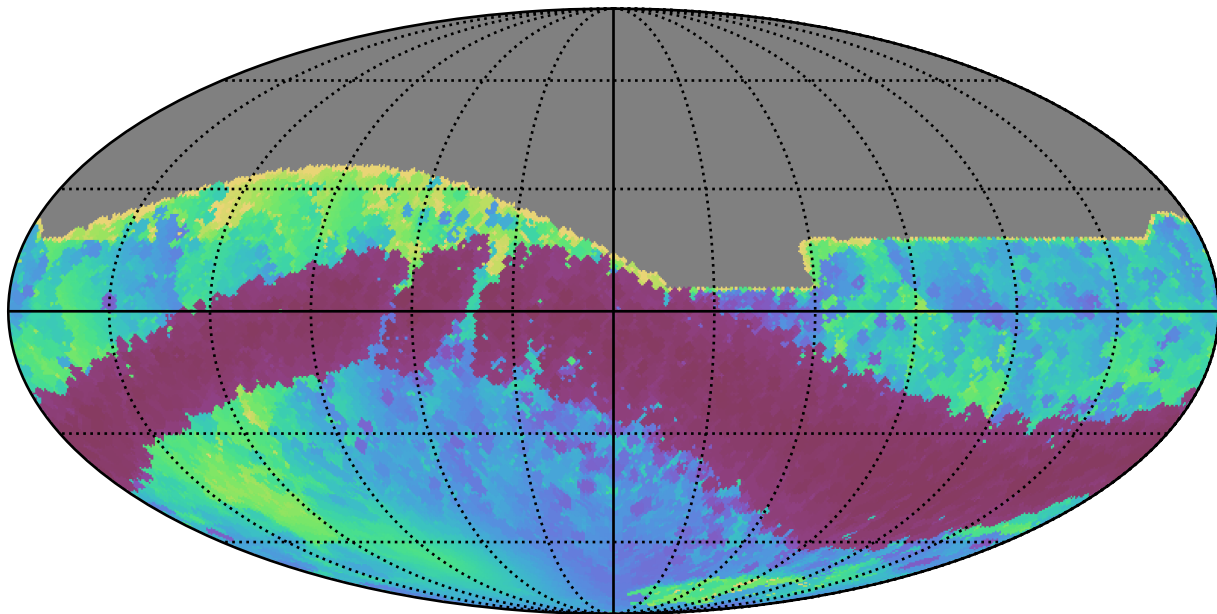
noroll_mjdp365_v3.4_10yrs All sky r band: Min solarElong
