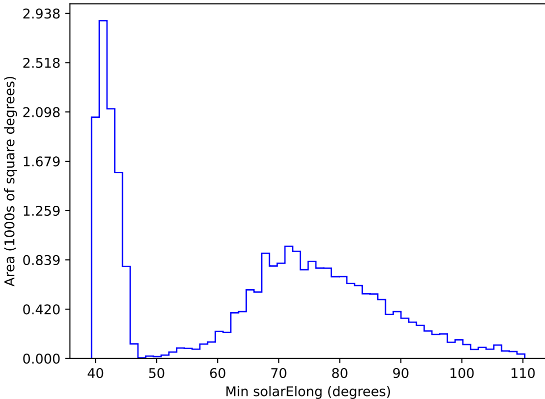
noroll_mjdp365_v3.4_10yrs All sky r band: Min solarElong
