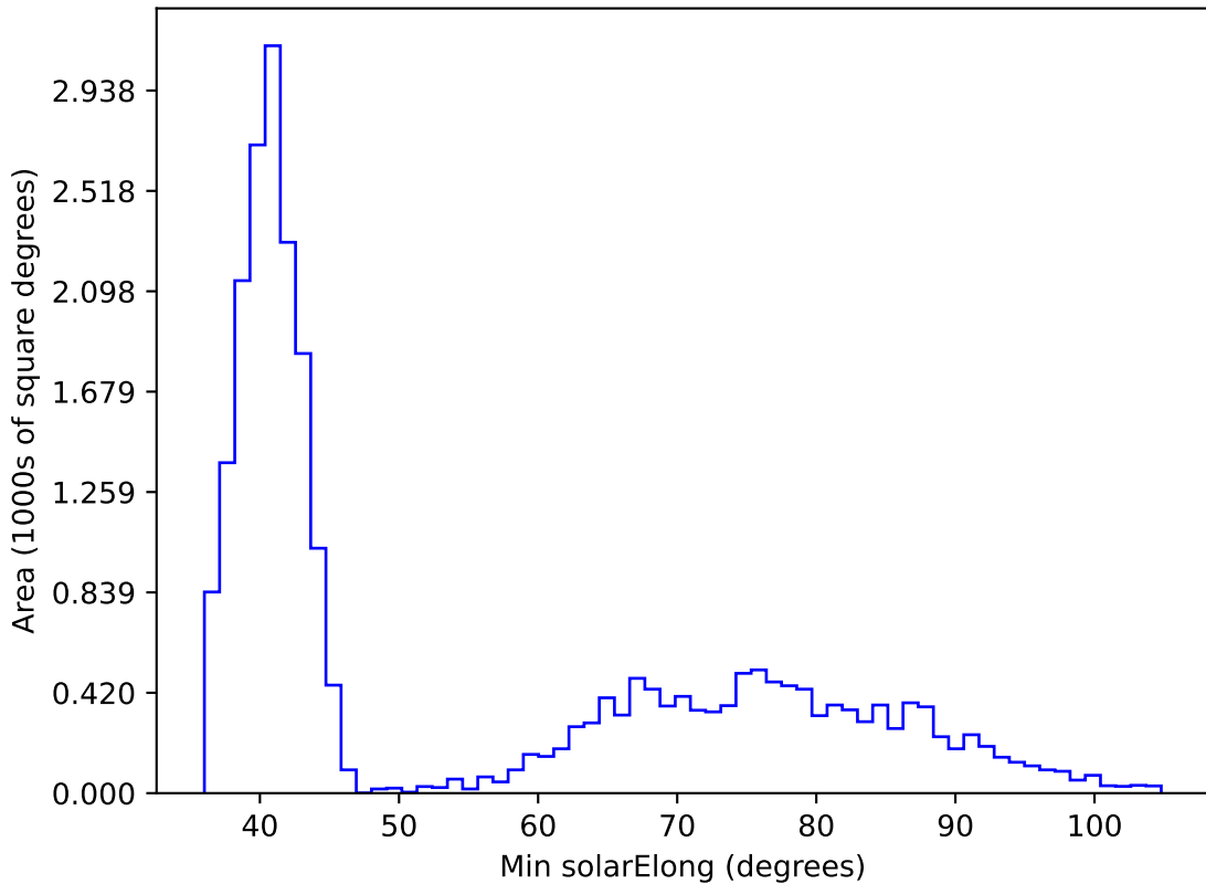
noroll_mjdp365_v3.4_10yrs All sky i band: Min solarElong
