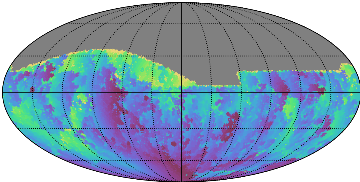
noroll_mjdp365_v3.4_10yrs All sky g band: Min solarElong
