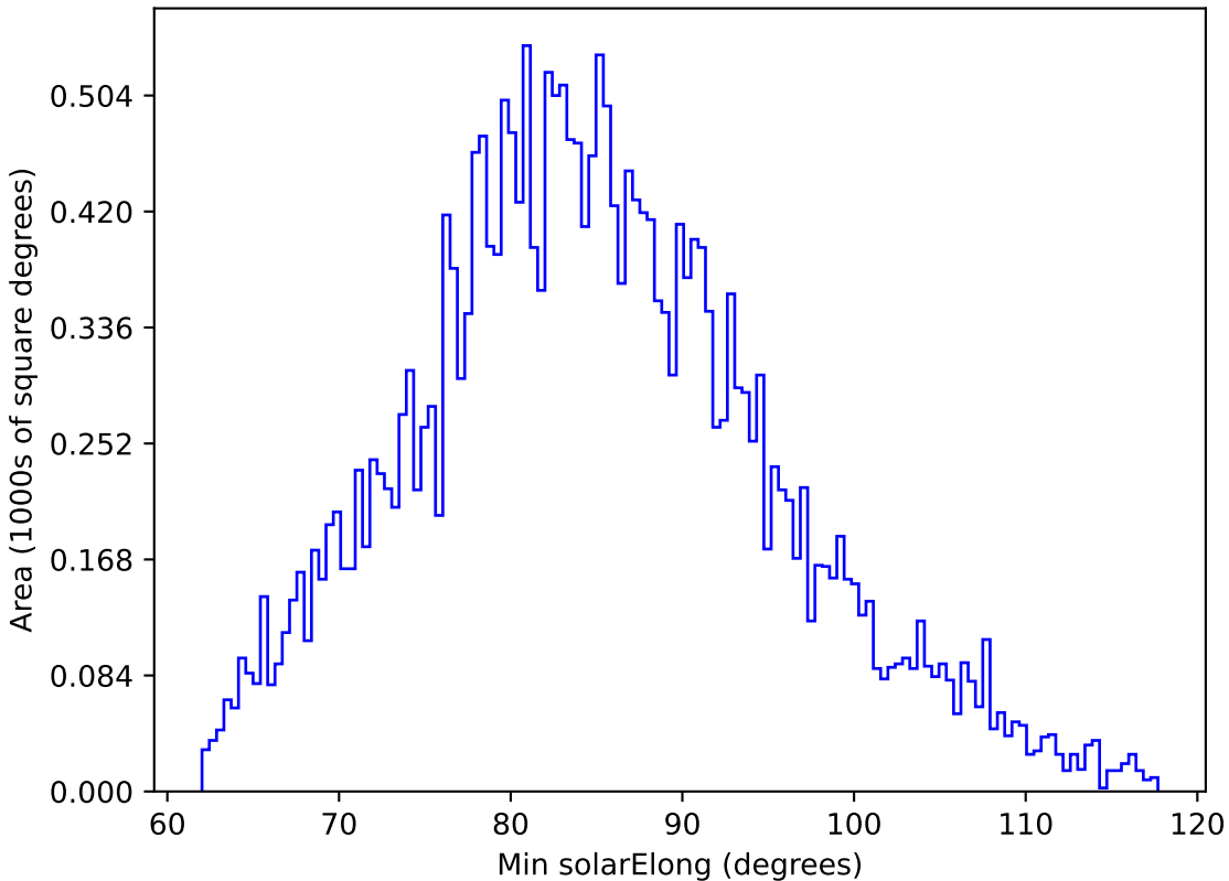
noroll_mjdp365_v3.4_10yrs All sky g band: Min solarElong
