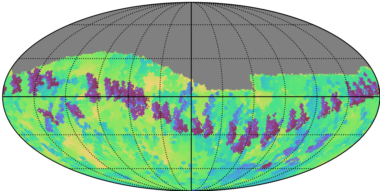
noroll_mjdp365_v3.4_10yrs Yr 1 z band: Min skyBrightness
