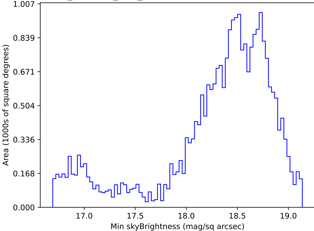
noroll_mjdp365_v3.4_10yrs Yr 1 z band: Min skyBrightness
