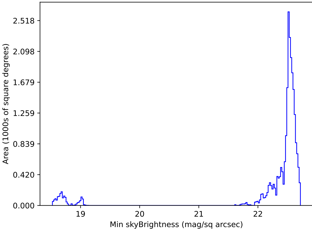
noroll_mjdp365_v3.4_10yrs Yr 1 u band: Min skyBrightness
