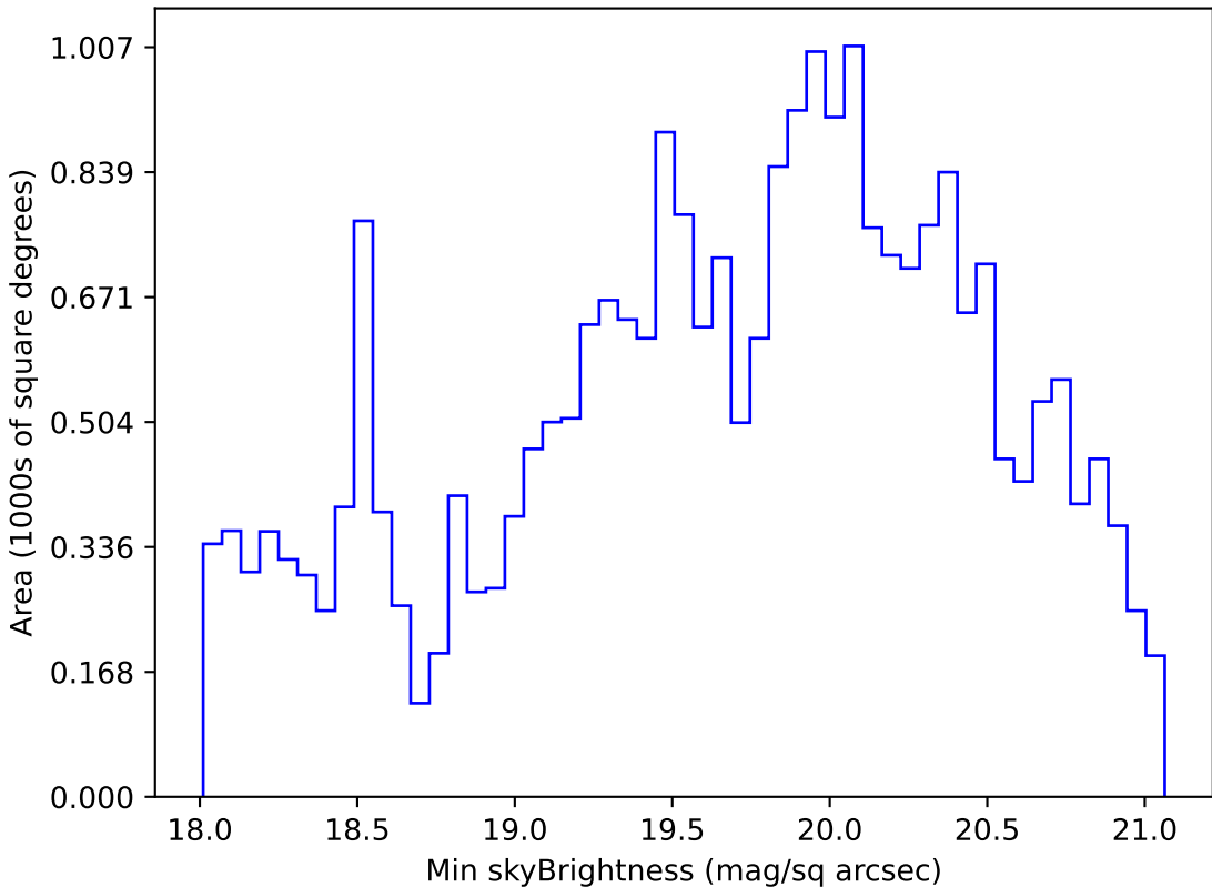
noroll_mjdp365_v3.4_10yrs Yr 1 r band: Min skyBrightness
