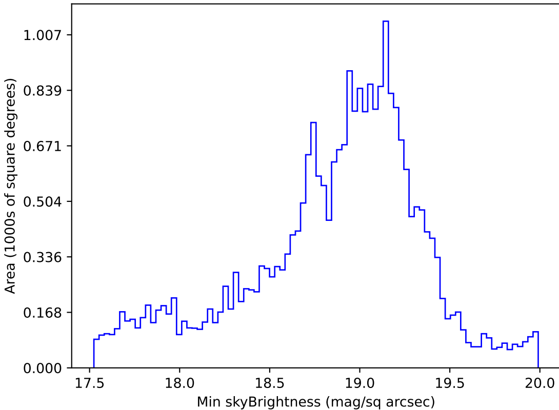
noroll_mjdp365_v3.4_10yrs Yr 1 i band: Min skyBrightness
