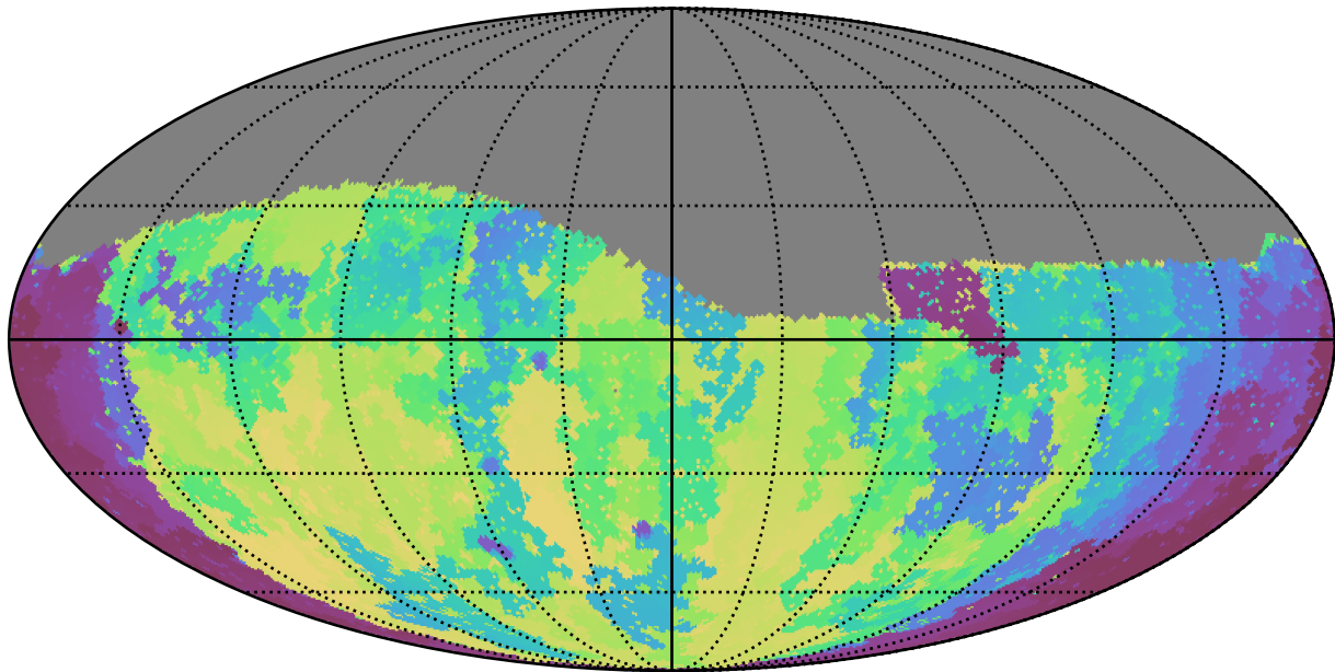
noroll_mjdp365_v3.4_10yrs Yr 1 g band: Min skyBrightness
