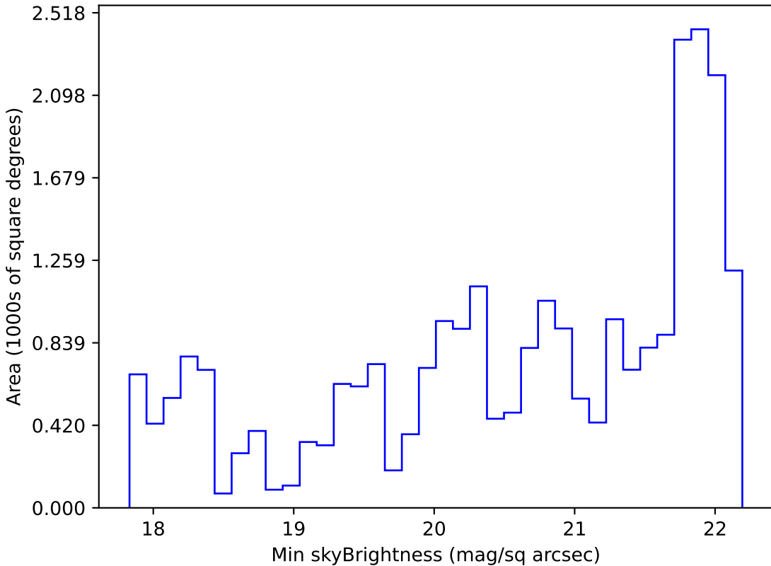
noroll_mjdp365_v3.4_10yrs Yr 1 g band: Min skyBrightness
