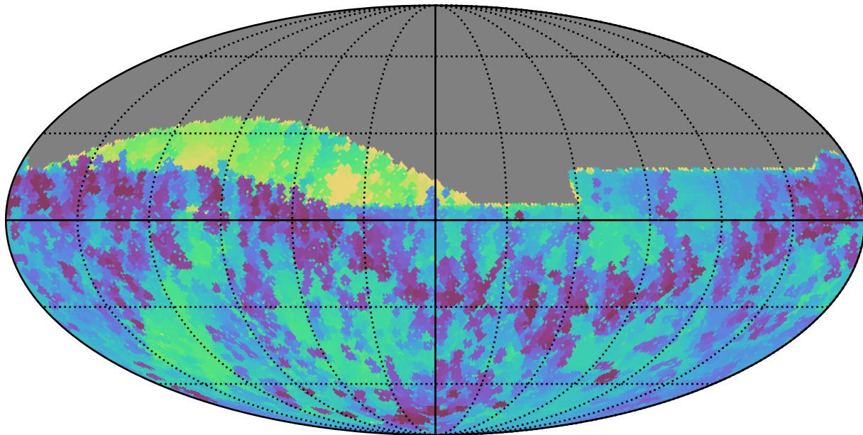
noroll_mjdp365_v3.4_10yrs Yr 1 all bands: Min skyBrightness
