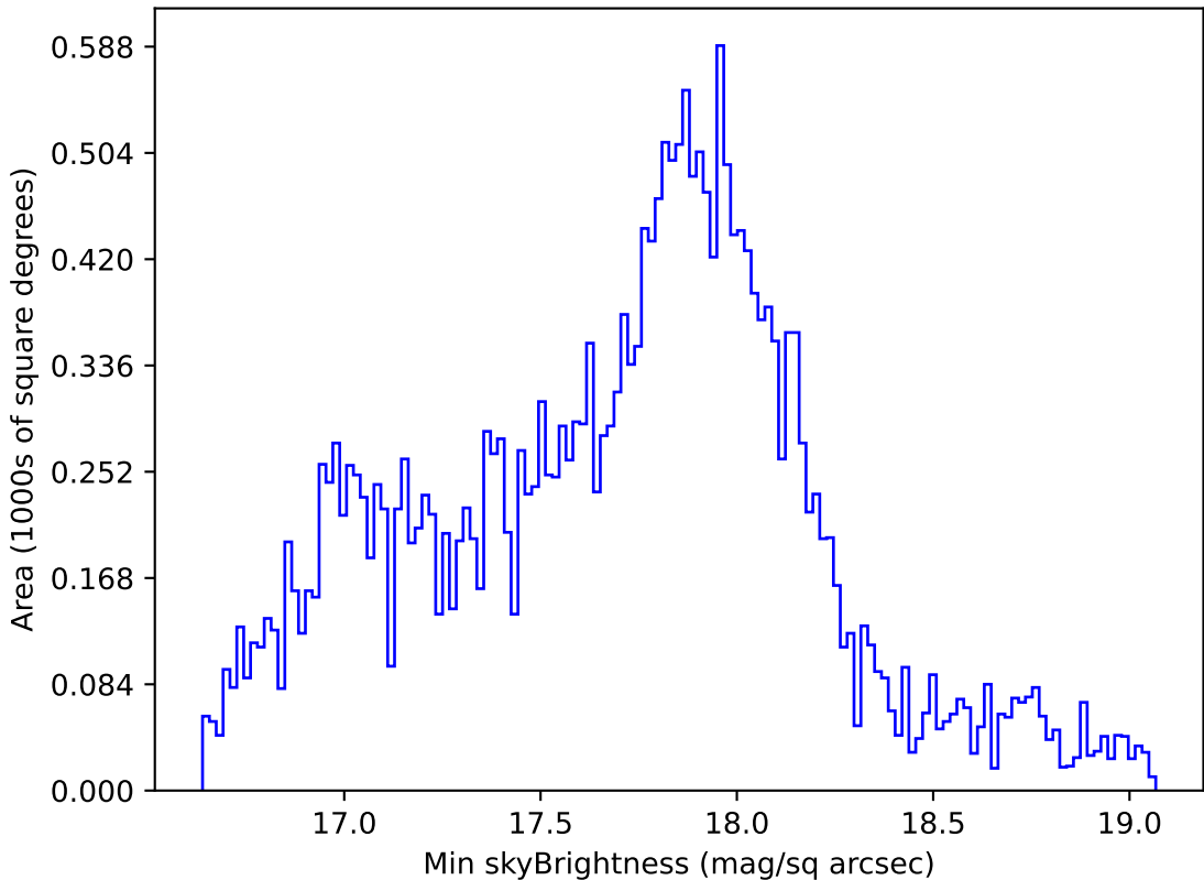
noroll_mjdp365_v3.4_10yrs Yr 1 all bands: Min skyBrightness
