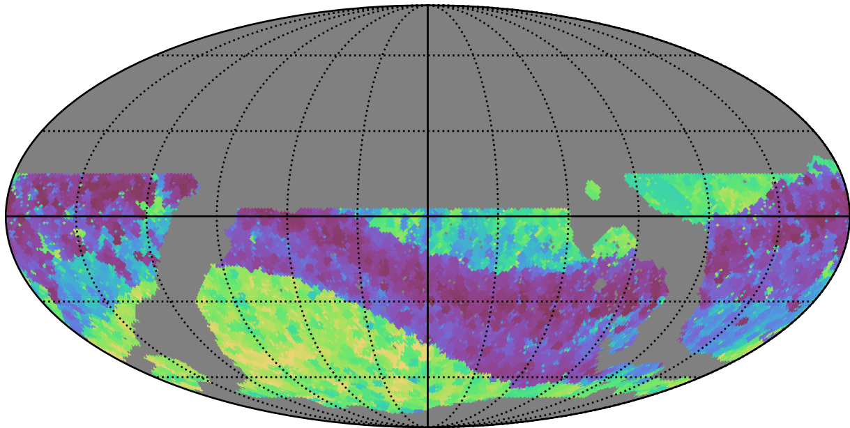
noroll_mjdp365_v3.4_10yrs WFD z band: Min skyBrightness
