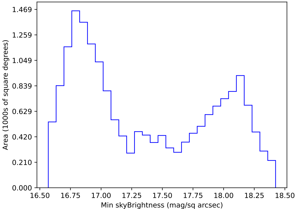
noroll_mjdp365_v3.4_10yrs WFD z band: Min skyBrightness
