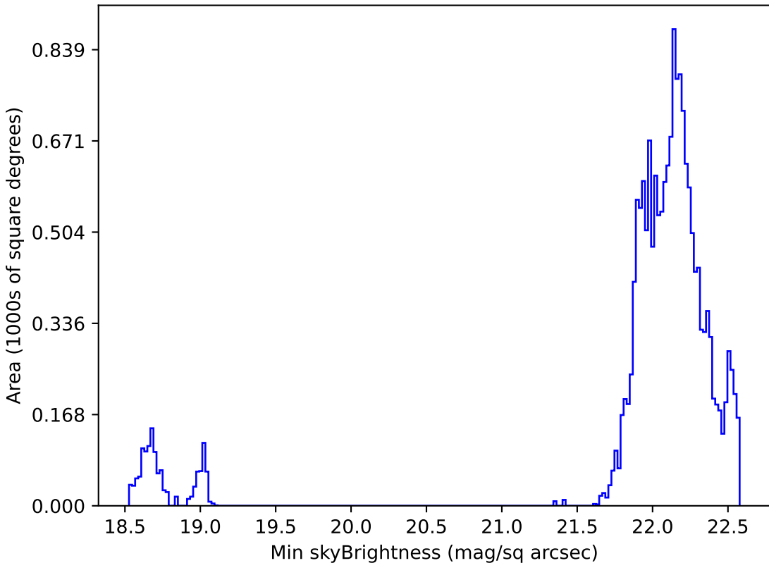
noroll_mjdp365_v3.4_10yrs WFD u band: Min skyBrightness
