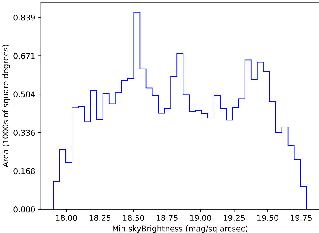
noroll_mjdp365_v3.4_10yrs WFD r band: Min skyBrightness
