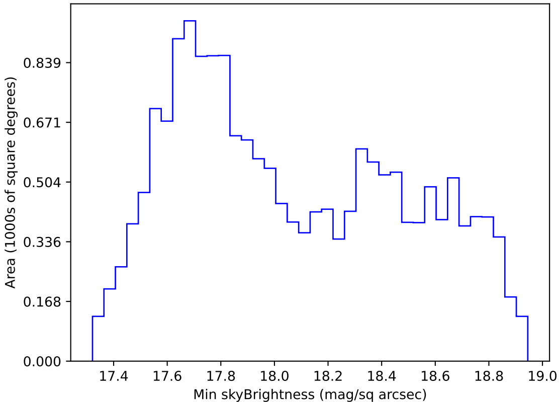
noroll_mjdp365_v3.4_10yrs WFD i band: Min skyBrightness
