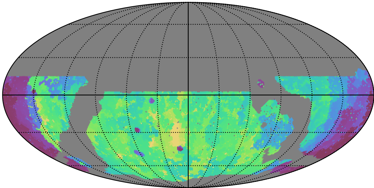
noroll_mjdp365_v3.4_10yrs WFD g band: Min skyBrightness
