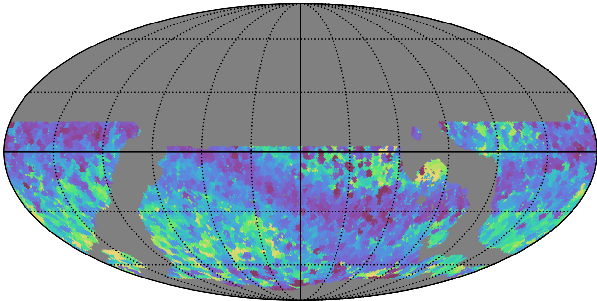
noroll_mjdp365_v3.4_10yrs WFD all bands: Min skyBrightness
