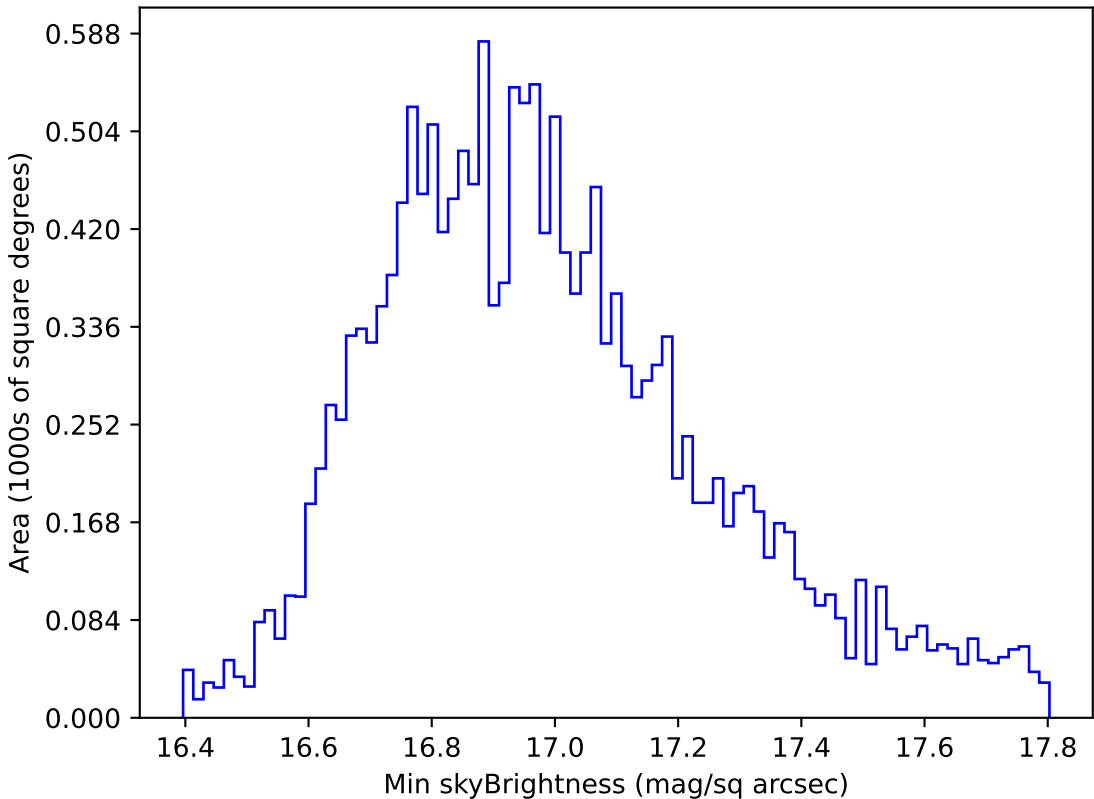
noroll_mjdp365_v3.4_10yrs WFD all bands: Min skyBrightness
