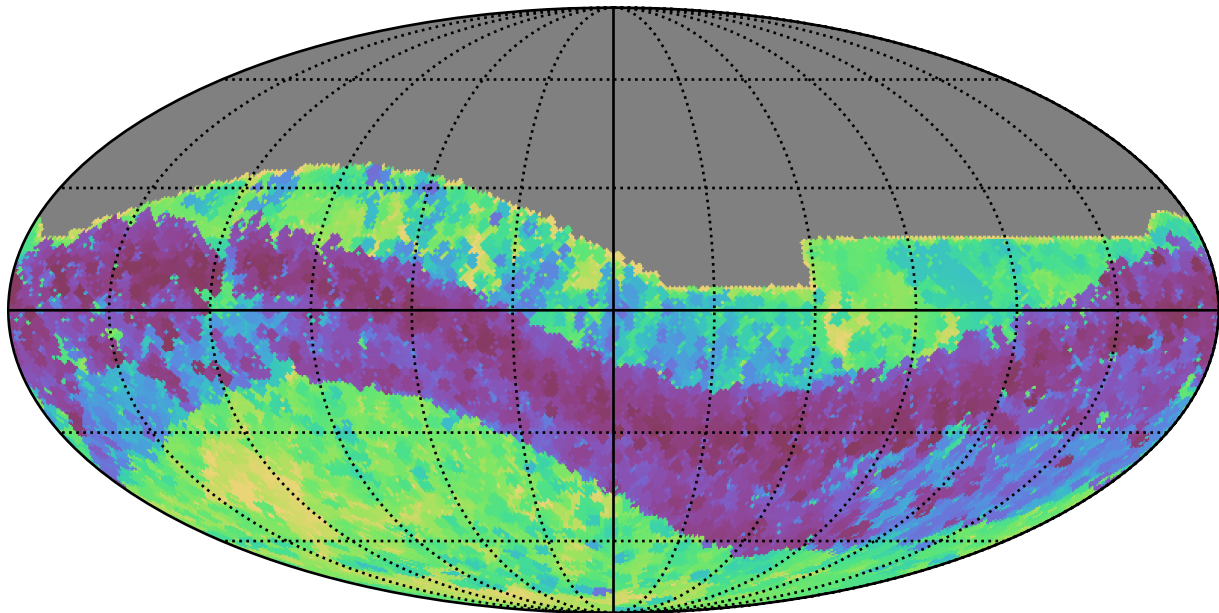
noroll_mjdp365_v3.4_10yrs All sky z band: Min skyBrightness
