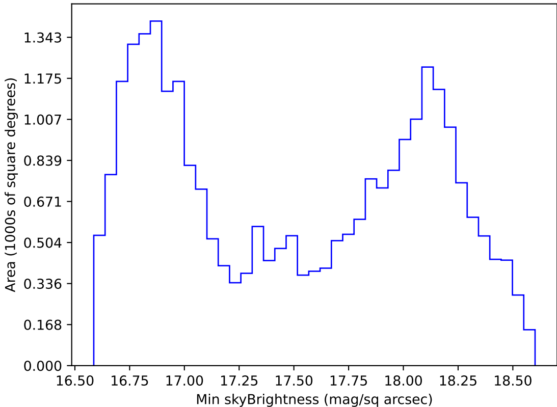
noroll_mjdp365_v3.4_10yrs All sky z band: Min skyBrightness
