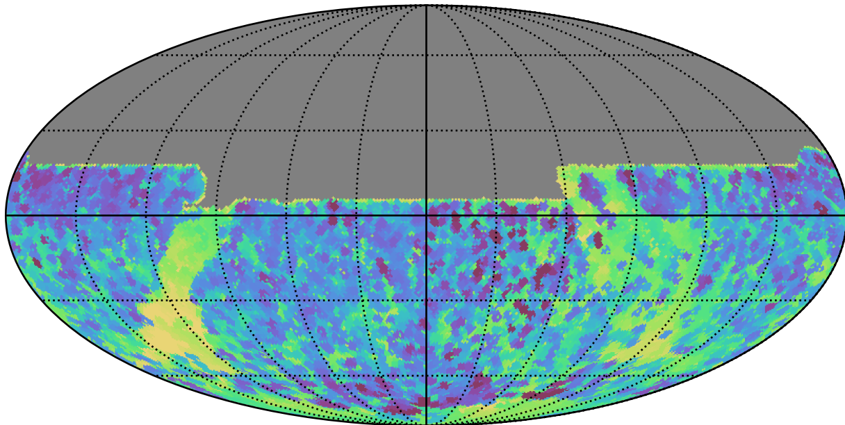
noroll_mjdp365_v3.4_10yrs All sky y band: Min skyBrightness
